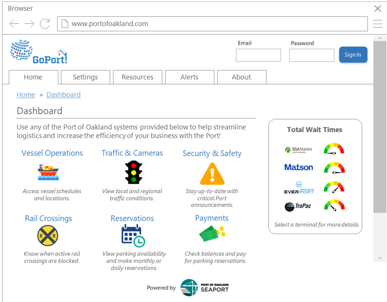
Figure 1: Website Home Screen Mock-Up
